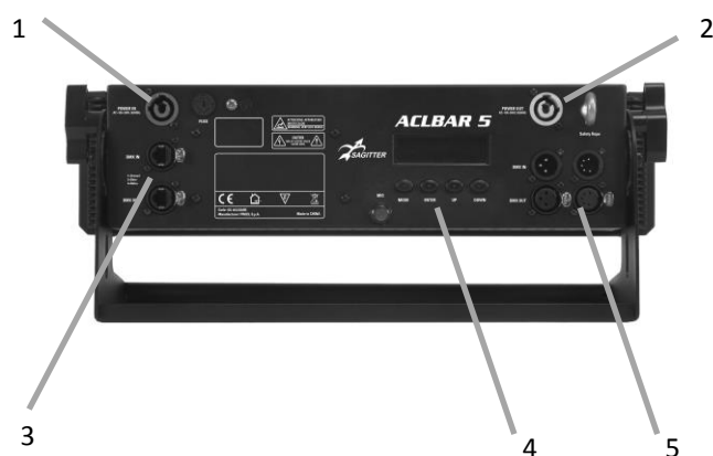
VISTA POSTERIORE 1 – Power IN 2 – Power OUT 3 - Artnet IN/OUT 4 - Display e pulsantiera 5 - 3/5 poli DMX IN / OUT
